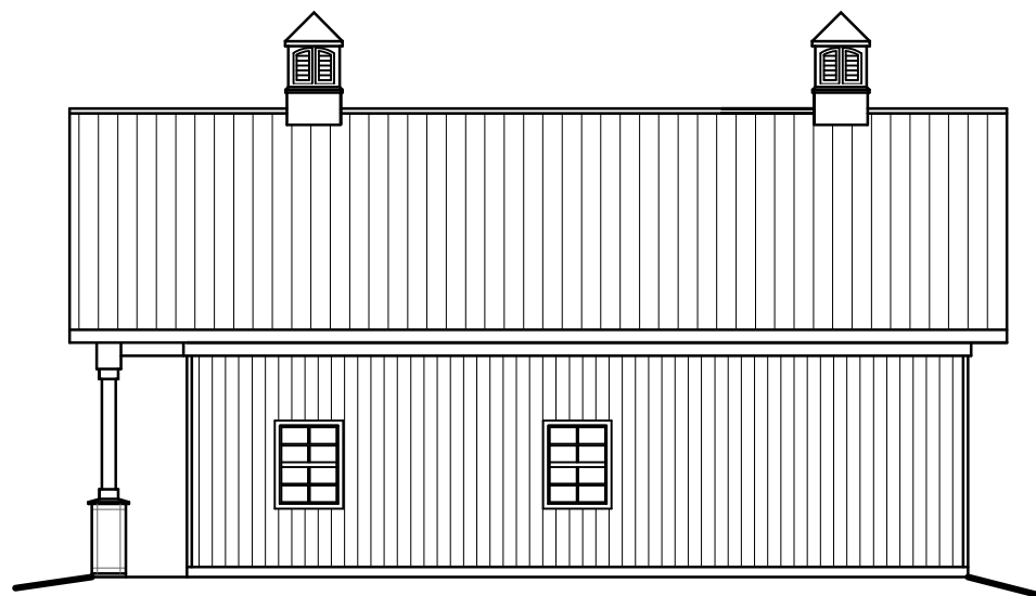
SOUTH ELEVATION: SCALE: 3/32" = 1'-0"
