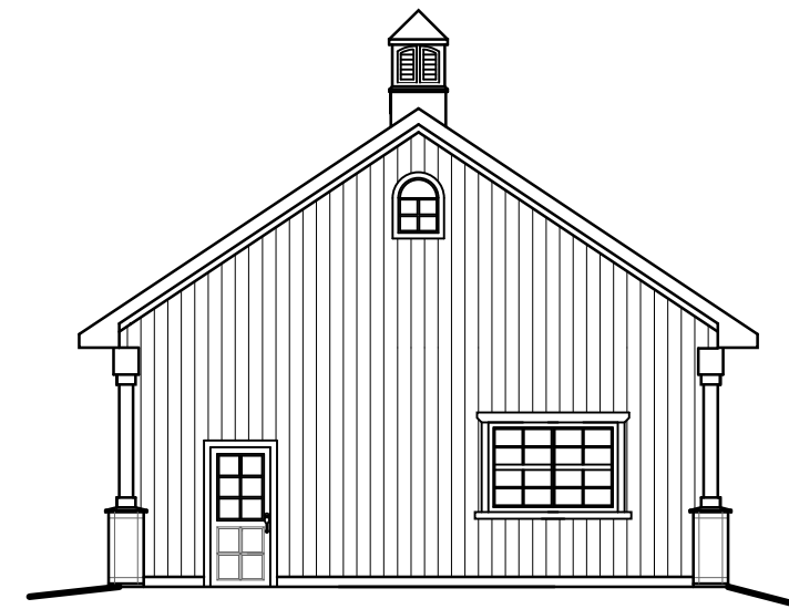
WEST ELEVATION: SCALE: 3/32" = 1'-0"
